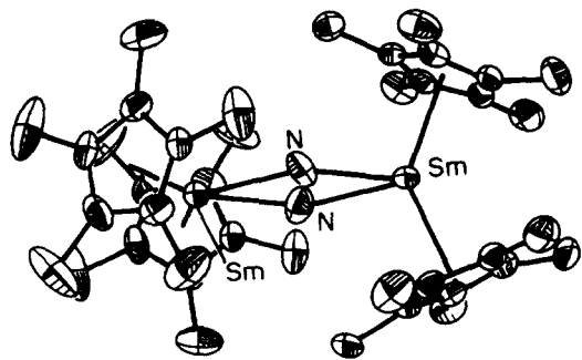
Fig. 16. [(C_5Me_5)_2Sm]_2(\mu-\eta^2:\eta^2-N_2) ( 29 ). (Reprinted with permission from the Journal of the American Chemical Society . The labelling has been simplified from that reported.)
