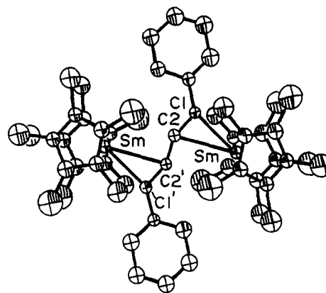
Fig. 6. [(C_5Me_5)_2Sm]_2(\mu-\eta^2:\eta^2-C_4Ph_2) ( 8 ). (Reprinted with permission from the Journal of the Chemical Society, Chemical Communications . The labelling has been simplified from that reported.)
