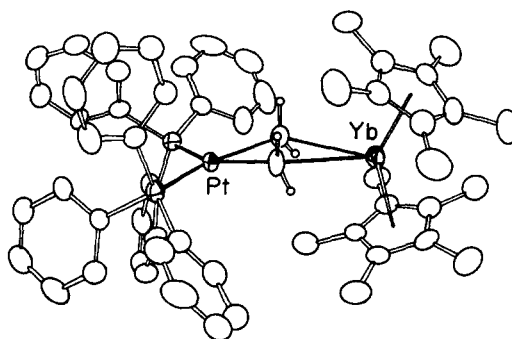
Fig. 1. (\text{Me}_5\text{C}_5)_2\text{Yb}(\mu\text{-C}_2\text{H}_4)\text{Pt}(\text{PPh}_3)_2 ( 1 ). (Reprinted with permission from the Journal of the American Chemical Society . The labelling has been simplified from that reported.)
