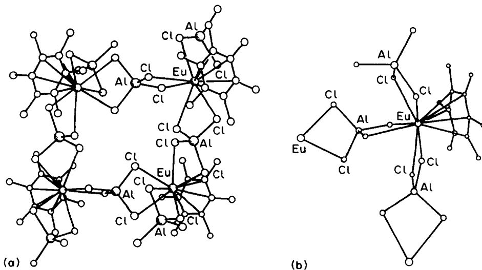
Fig. 11. [\text{Eu}(\text{C}_6\text{Me}_6)(\text{AlCl}_4)_2]_4 ( 16 ): (a) the tetrameric unit; (b) the \text{Eu} environment. ((a) Reprinted with permission from Journal of the Chemical Society, Chemical Communications . The labelling has been simplified from that reported.)
