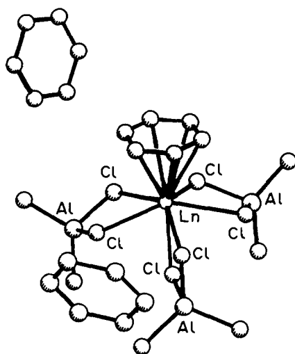
Fig. 8. [\text{Ln}(\eta^6\text{-C}_6\text{H}_6)(\text{AlCl}_4)_3 \cdot \text{C}_6\text{H}_6 ( \text{Ln} = \text{Nd} (11) or \text{Sm} (12)). (Reprinted with permission from the Journal of Organometallic Chemistry . The labelling has been simplified from that reported.)
