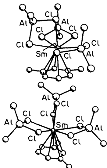
Fig. 10. \text{Sm}(\eta^6\text{-}m\text{-(CH}_3)_2\text{C}_6\text{H}_4)(\text{AlCl}_4)_3 ( 15 ). (Reprinted with permission from the Journal of Organometallic Chemistry . The labelling has been simplified from that reported.)
