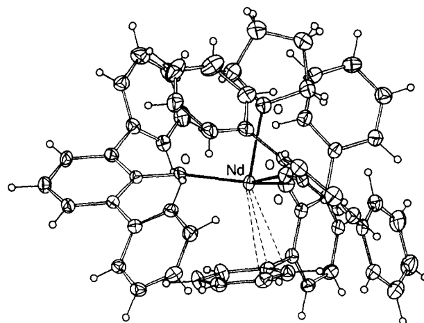
Fig. 14. Nd(Odpp) 3 (THF) ( 23 ). (Reprinted with permission from the Australian Journal of Chemistry . The labelling has been simplified from that reported.)
