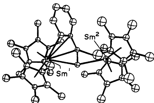
Fig. 4. [(C_5Me_5)_2Sm]_2(\mu-\eta^2:\eta^4-CH_2CHPh) ( 5 ). (Reprinted with permission from the Journal of the American Chemical Society . The labelling has been simplified from that reported.)
