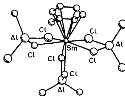
Fig. 9. \text{Sm}(\eta^6\text{-CH}_3\text{C}_6\text{H}_5)(\text{AlCl}_4)_3 (14). (Reprinted with permission from Youji Huaxue . The labelling has been simplified from that reported.)
