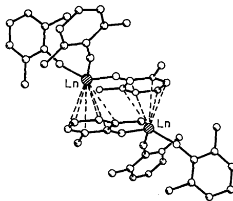
Fig. 15. The X-ray structure of [\text{Ln}(\text{OC}_6\text{H}_3^i\text{Pr}_2-2,6)_2(\mu-(\text{OC}_6\text{H}_3^i\text{Pr}_2-2,6)-\text{O}:\eta^6)]_2 \text{Ln} = \text{Nd} ( 25 ) or \text{Sm} ( 26 ). (Reprinted with permission from Inorganic Chemistry . The labelling has been simplified from that reported.)
