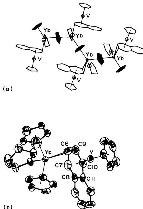
Fig. 3. The molecular structure of [(\eta^5\text{-Cp})\text{V}(\mu\text{-}\eta^6\text{:}\eta^2\text{-C}_{10}\text{H}_8)\text{Yb}(\mu\text{-}\eta^5\text{:}\eta^5\text{-Cp})(\text{THF})]_n ( 3 ) (a) showing the [\text{Yb}(\mu\text{-}\eta^5\text{:}\eta^5\text{-Cp})]_n^+ zigzag chain and (b) showing the Yb coordination environment. (Reprinted with permission from Inorganica Chimica Acta . The labelling has been simplified from that reported.)
