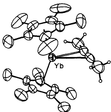
Fig. 5. (Me_5C_5)_2Yb(\eta^2-MeC\equiv CMe) ( 7 ). (Reprinted with permission from the Journal of the American Chemical Society . The labelling has been simplified from that reported.)
