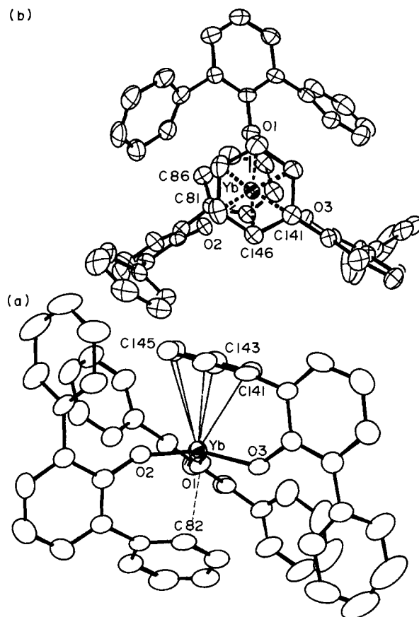
Fig. 13. \text{Yb}(\text{Odpp})_3 (19) (a) showing the coordination sphere and (b) showing the pseudotwo-fold axis along \text{Yb}-\text{O}(1) . (Reprinted with permission from the Australian Journal of Chemistry . The labelling has been simplified from that reported.)
