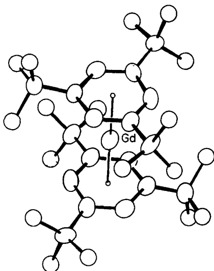
Fig. 12. [\text{Gd}(\eta^6\text{-}^t\text{Bu}_3\text{C}_6\text{H}_3)_2] (17). (Reprinted with permission from the Journal of the Chemical Society, Chemical Communications . The labelling has been simplified from that reported.)
