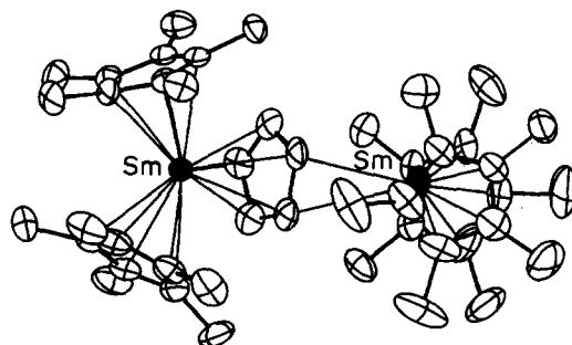
Fig. 2. (\text{C}_5\text{Me}_5)_2\text{Sm}(\mu\text{-C}_5\text{H}_5)\text{Sm}(\text{C}_5\text{Me}_5)_2 ( 2 ). (Reprinted with permission from the Journal of the American Chemical Society . The labelling has been simplified from that reported.)
