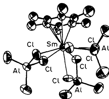
Fig. 7. \text{Sm}(\eta^6\text{-C}_6\text{Me}_6)(\text{AlCl}_4)_3 ( 10 ). (Reprinted with permission from the Journal of the American Chemical Society . The labelling has been simplified from that reported.)
